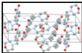
Fig. 2. Packing diagram of the title compound showing the intermolecular interaction (dashed lines) between nitro group atom O3 and benzene ring C1-C6 (centroid indicated by pink sphere).
